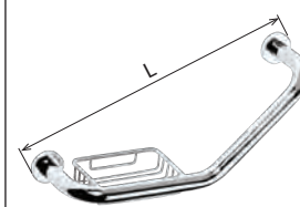
Madlo lomené s mýdlenkou Bath grab bar angular with soap basket 400 x 250 x 135 mm 102307032
